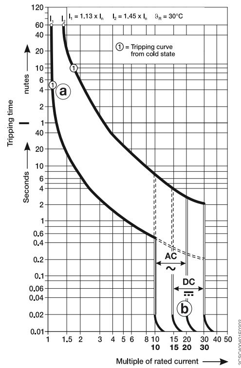
Characteristic D IEC-EN60898
