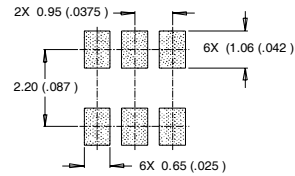
RECOMMENDED FOOTPRINT
