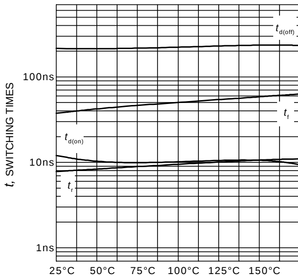
Figure 11. Typical switching times as a function of junction temperature (inductive load, V_{CE} = 400\text{V} , V_{GE} = 0/15\text{V} , I_C = 10\text{A} , r_G=23\Omega , Dynamic test circuit in Figure E)
