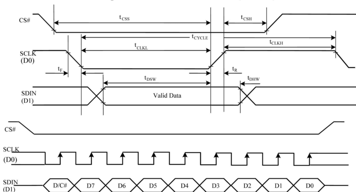
Figure 13-4: Serial interface characteristics (3-wire SPI)
