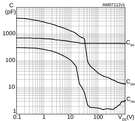
Figure 8: Capacitance variations
