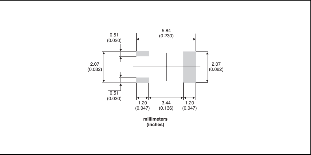
Figure 15. SMBflat-3L footprint dimensions
