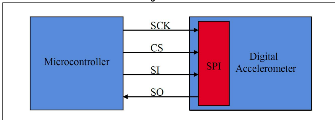
Figure 22. SPI
