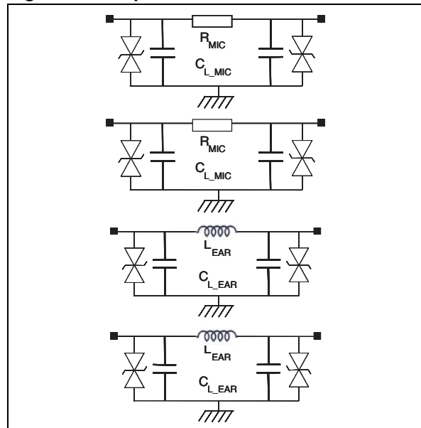
Figure 2. Equivalent circuit
