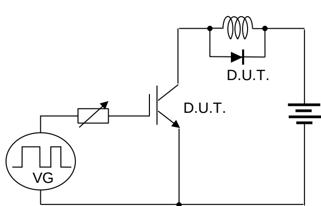
Fig.23 Inductive Load Circuit
