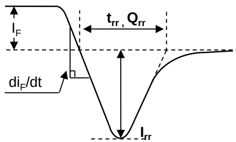
Fig.25 Diode Reverce Recovery Waveform
