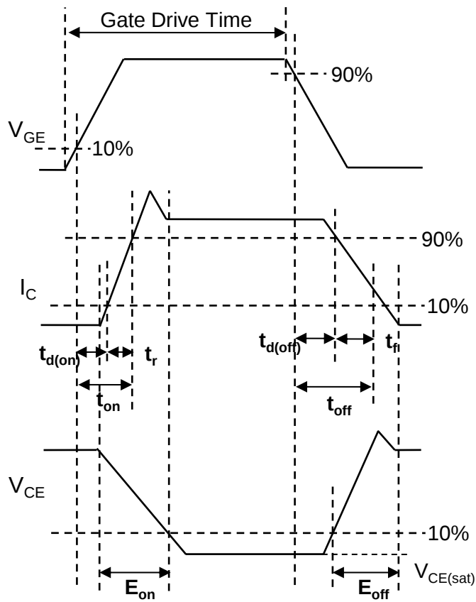
Fig.19 Inductive Load Waveform
