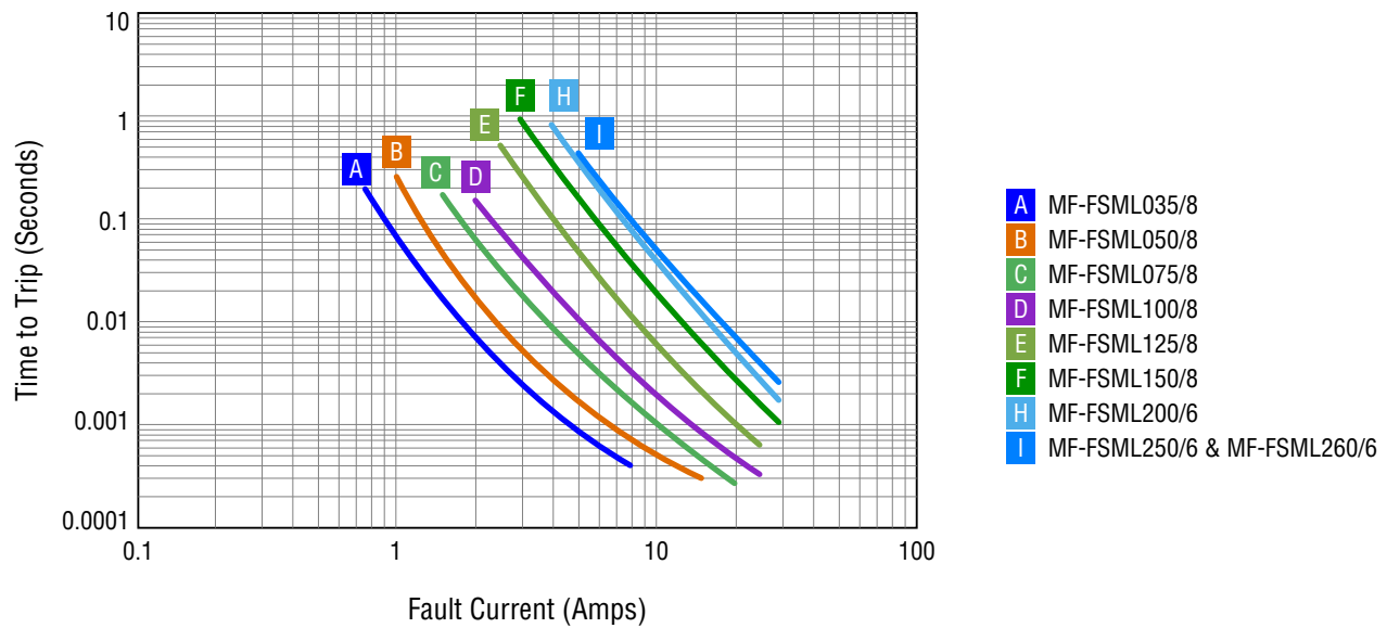
Typical Time to Trip at 23 °C
