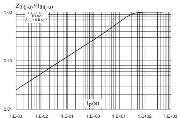
Figure 4. Relative variation of thermal impedance junction to ambient versus pulse duration (PCB FR4, copper thickness = 35 µm, S CU = 0.5 cm 2 )(TO-92)
