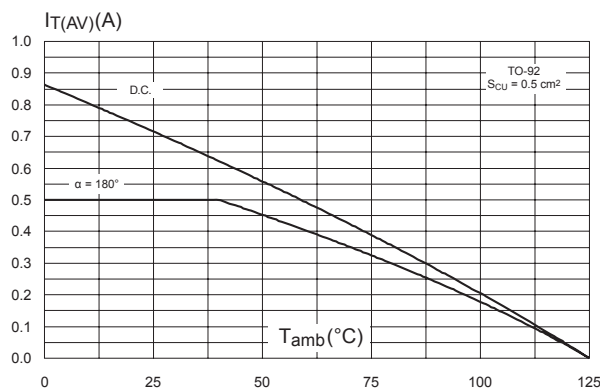
Figure 3. Average and DC on-state current versus ambient temperature (epoxy printed circuit board FR4, copper thickness = 35 µm, S CU = 0.5 cm 2 )(TO-92)
