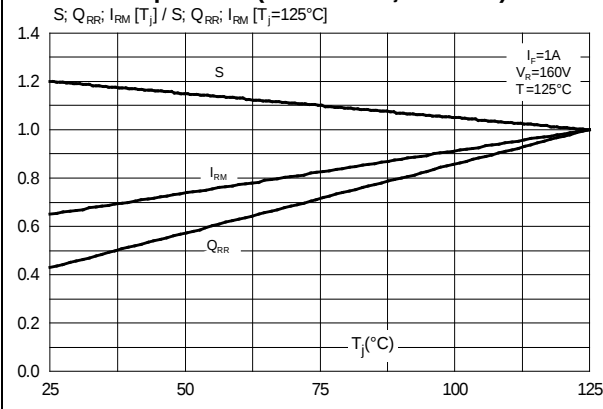
Figure 9: Dynamic parameters versus junction temperature (reference T_J = 125^\circ C )
