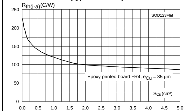
Figure 11: Thermal resistance junction to ambient total versus copper surface under each lead (typical values)
