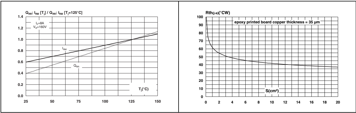
Figure 9. Dynamic parameters versus junction temperature Figure 10. Thermal resistance, junction to ambient, versus copper surface area under tab
