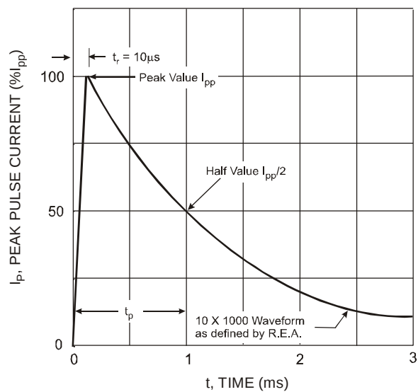
Fig. 4 Pulse Waveform
