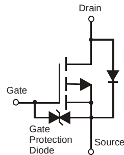
Internal Schematic
