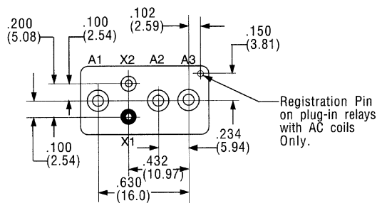
TERMINAL VIEW
