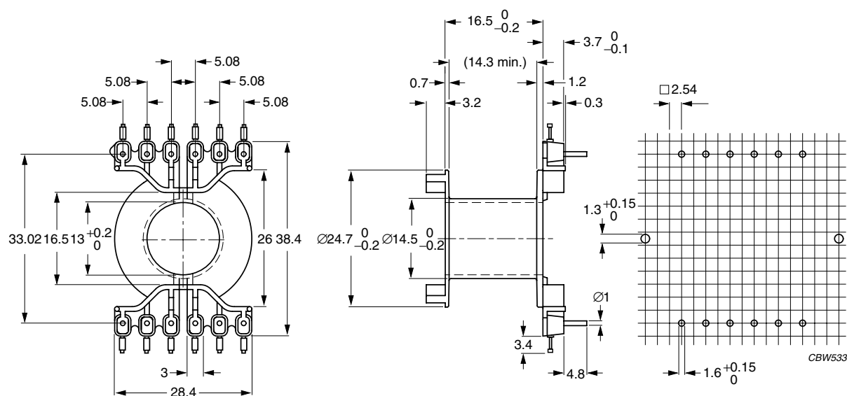
Fig.2 RM12/I coil former (DIL).
