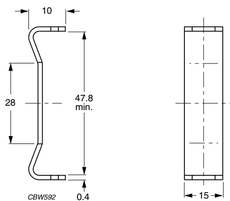
Fig.3 Mounting clip for ETD44/22/15.
