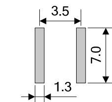
Recommended Pad Size
