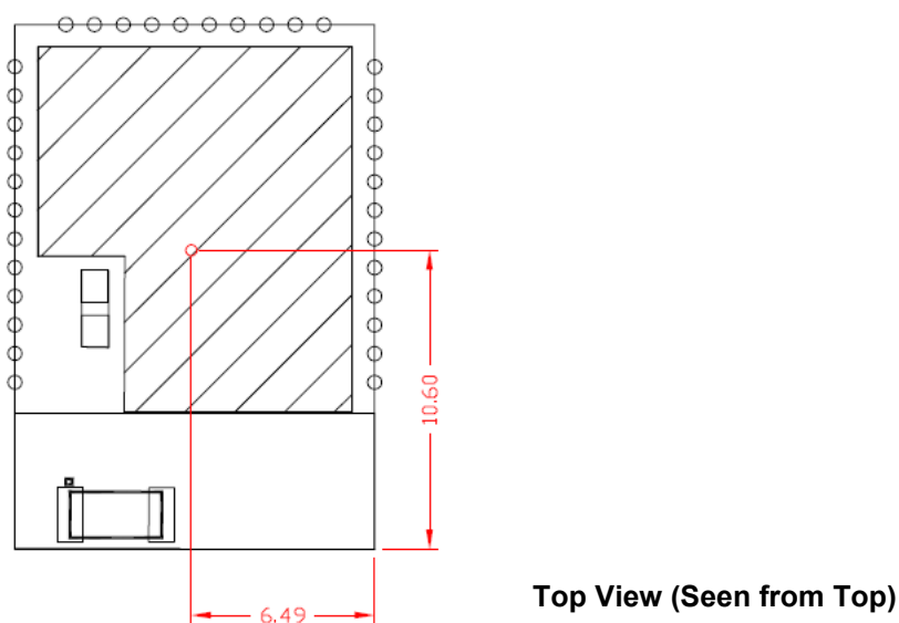
Figure 23. CYBT-483039-02 Center of Mass
