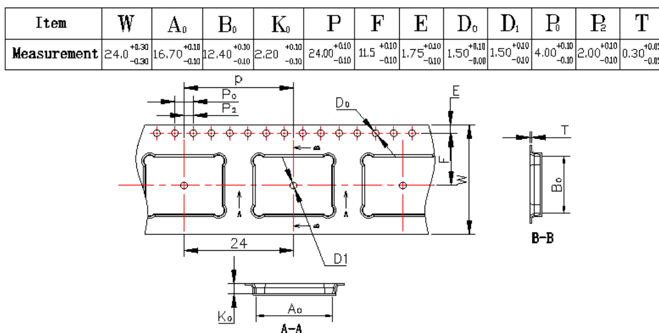
Figure 20. CYBT-413034-02 Tape Dimensions
