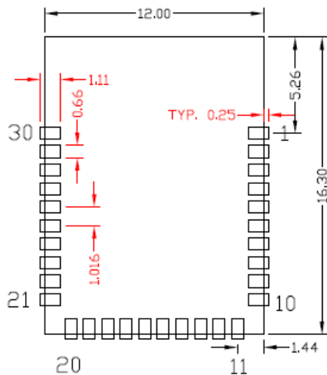
Figure 5. CYBT-413034-02 Host Layout (Dimensioned)
