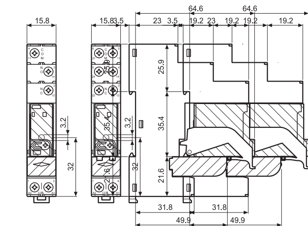
Types 4C.01 / 4C.02 Screw terminals
