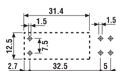
45.91...0310 (1 NO/SPST-NO)
