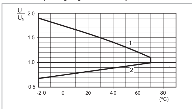
R 7S - DC coil operating range v ambient temperature - 7S.43/63
