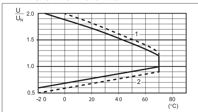
R 7S - DC coil operating range v ambient temperature - 7S.12/32 / 7S.23 / 7S.14/34 / 7S.16/36
