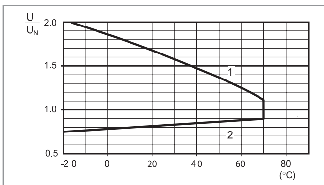
R 7S - AC coil operating range v ambient temperature - 7S.12/32 / 7S.14/34 / 7S.16/36
