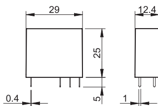
Types 50.12...1000/50.12...5000
