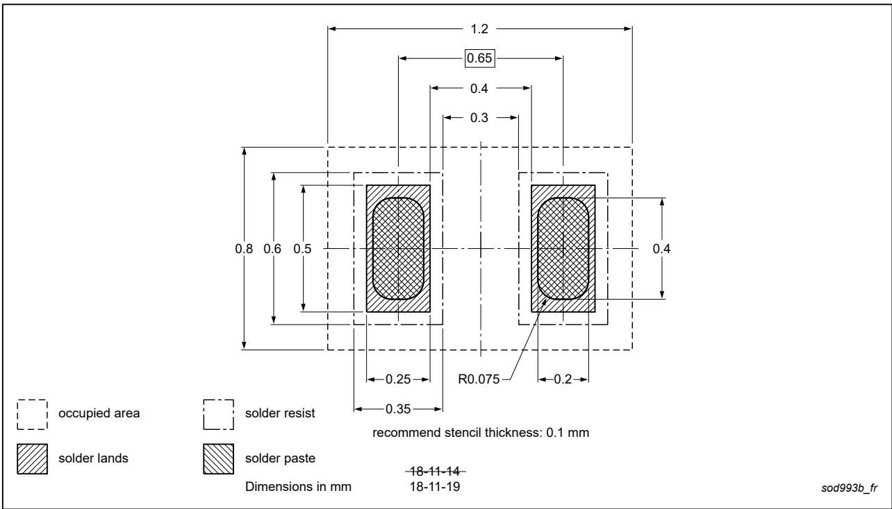
Fig. 14. Reflow soldering footprint for DSN1006-2 (SOD993B)
