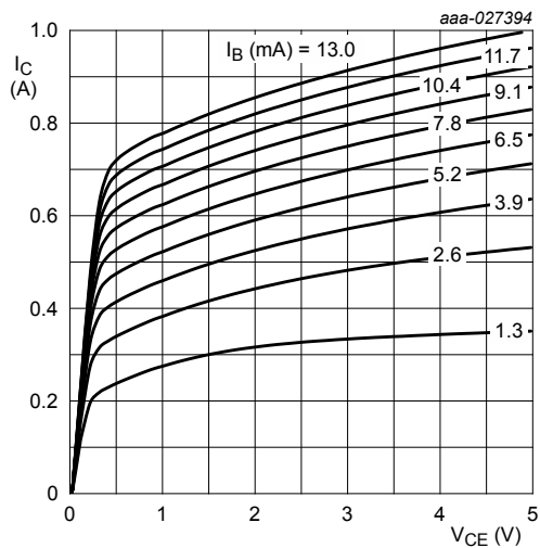
T_{amb} = 25\text{ }^{\circ}\text{C} Figure 39. BC817K-40H: Collector current as a function of collector-emitter voltage; typical values
