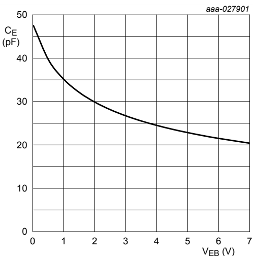
f = 1\text{ MHz} ; T_{amb} = 25\text{ }^{\circ}\text{C} Figure 41. BC817K-40H: Emitter capacitance as a function of emitter-base voltage; typical values
