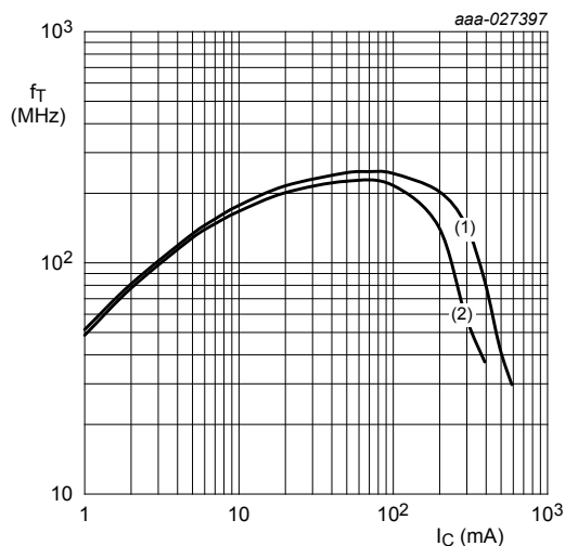
f = 100\text{ MHz} ; T_{amb} = 25\text{ }^{\circ}\text{C} (1) V_{CE} = 5\text{ V} (2) V_{CE} = 1\text{ V} Figure 42. BC817K-40H: Transition frequency as a function of collector current voltage; typical values
