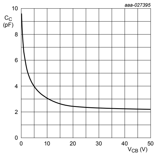
f = 1\text{ MHz} ; T_{amb} = 25\text{ }^{\circ}\text{C} Figure 40. BC817K-40H: Collector capacitance as a function of collector-base voltage; typical values
