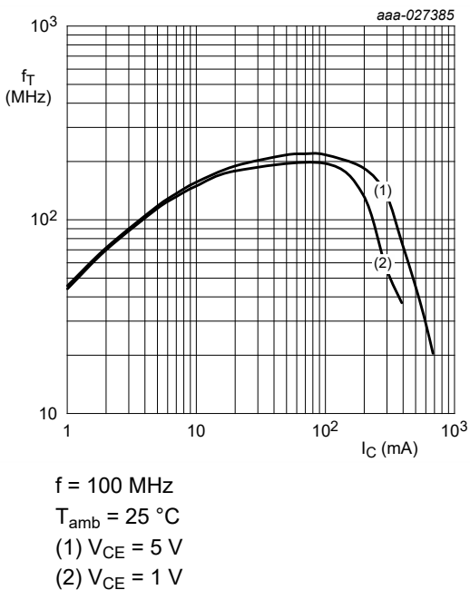
Fig. 30. BC817K-25H: Transition frequency as a function of collector current; typical values
