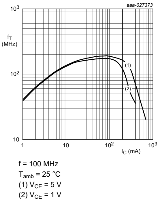
Fig. 18. BC817K-16H: Transition frequency as a function of collector current; typical values
