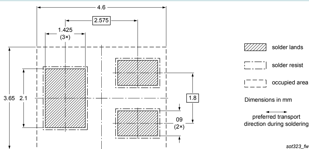
Figure 21. Wave soldering footprint for SOT323 (SC-70)
