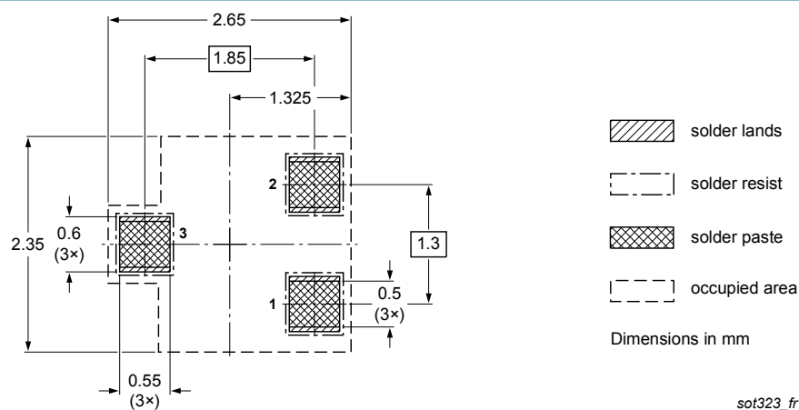
Figure 20. Reflow soldering footprint for SOT323 (SC-70)
