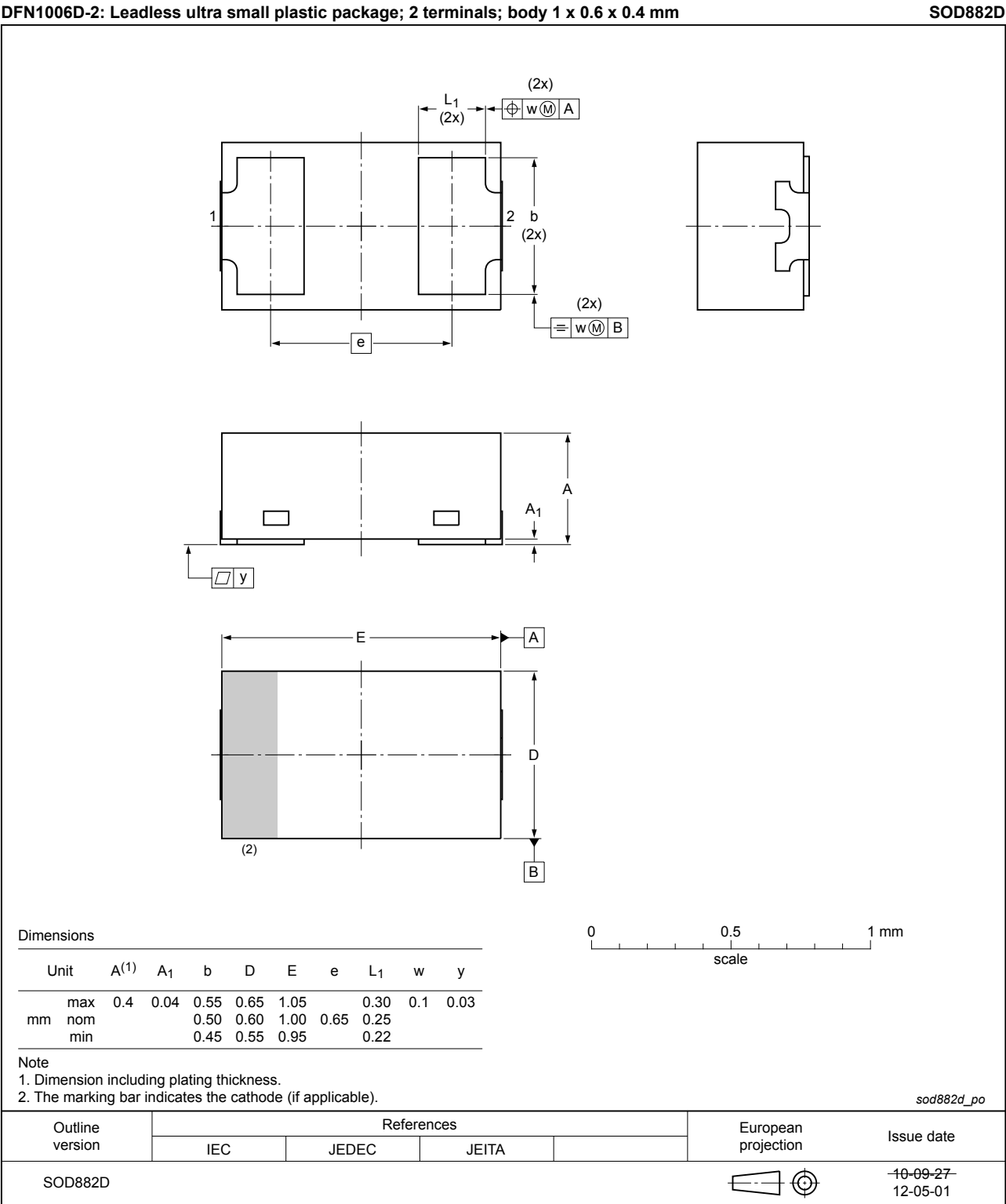
Fig. 10. Package outline DFN1006D-2 (SOD882D)
