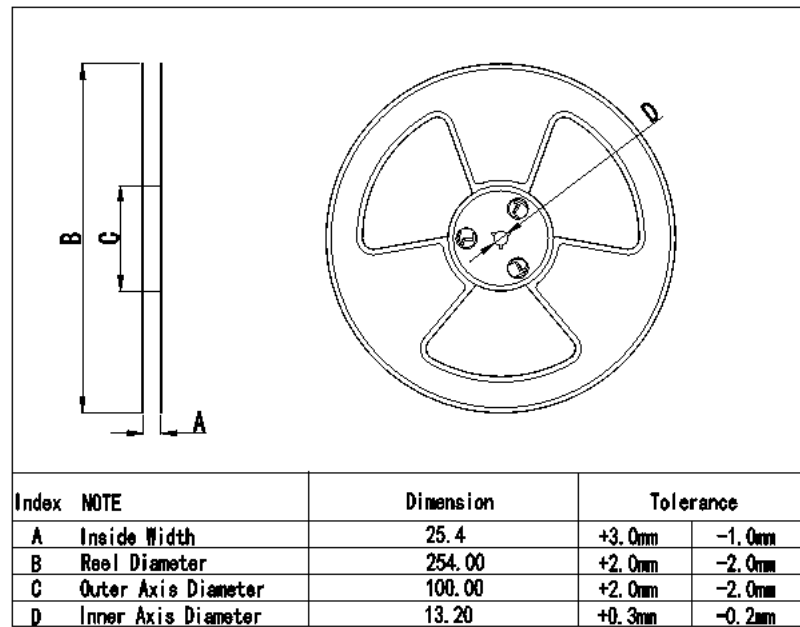
Figure 13. Reel Dimensions
