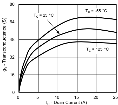
Transconductance
