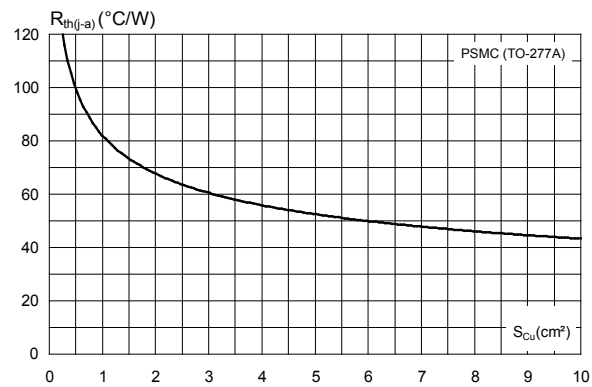
Figure 7. Thermal resistance junction to ambient versus copper surface under tab (typical values, epoxy printed board FR4, e_{Cu} = 35\ \mu\text{m} ) (PSMC (TO-277A))
