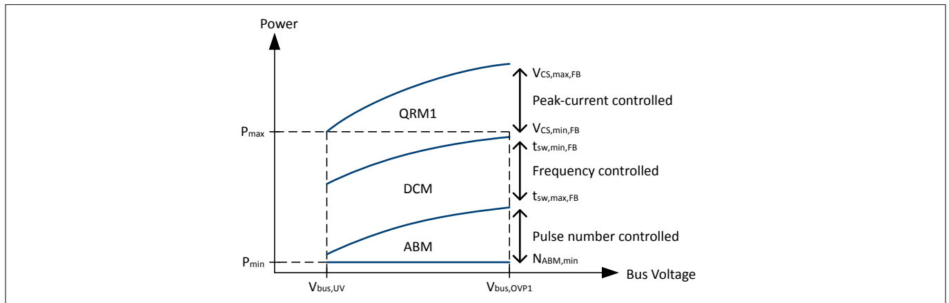
Figure 21 Flyback Multimode Operation Scheme
