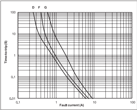
Typical Time-To-Trip at 23°C
