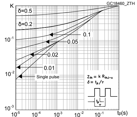
Figure 2. Thermal impedance
