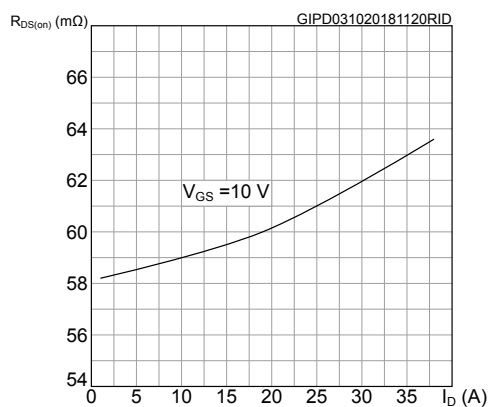
Figure 5. Static drain-source on resistance
