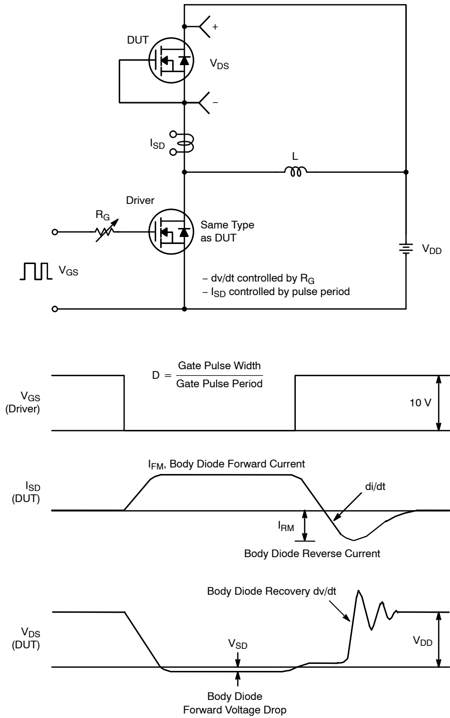
Figure 22. Peak Diode Recovery d v / d t Test Circuit & Waveforms
