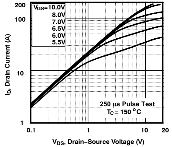
Figure 2. On-Region Characteristics
