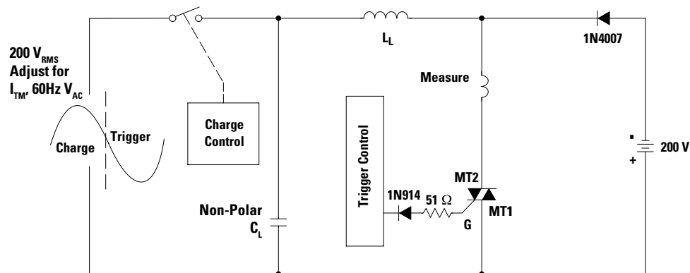
Figure 16. Simplified Test Circuit to Measure the Critical Rate of Rise of Commutating Current (di/dt)
