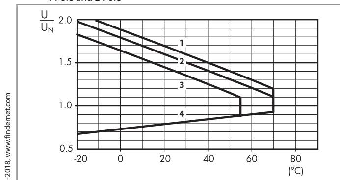
R 38 - DC coil operating range v ambient temperature
