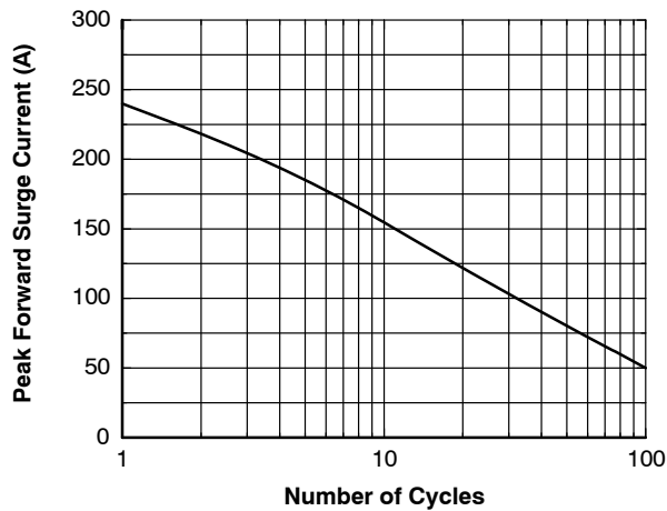
Figure 7. Maximum Non-Repetitive Peak Forward Surge Current
