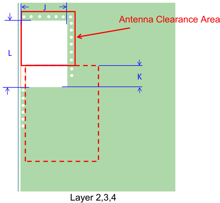
Fig 10. QN9080-001-M17 module on 36 mm x 31 mm GND PCB layout guide - center edge - clearance area layers 2, 3, 4 dimensions
