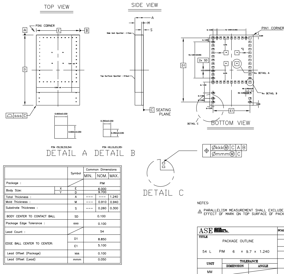
Fig 5. Footprint information for reflow soldering of SIPs
