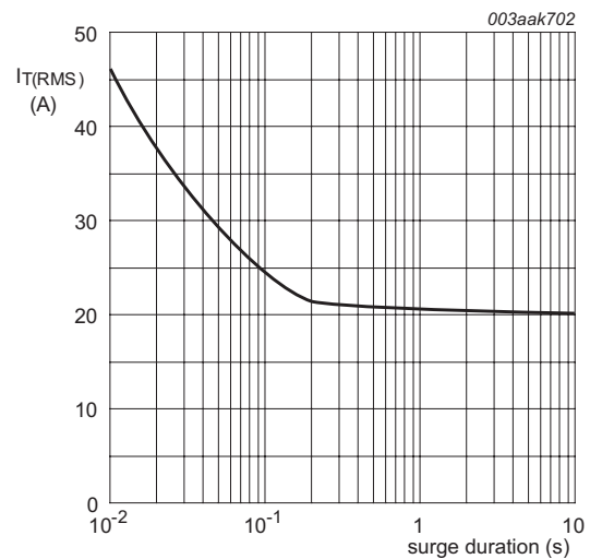
Fig. 2. RMS on-state current as a function of surge duration; maximum values f = 50\text{ Hz} ; T_{\text{mb}} = 122\text{ }^{\circ}\text{C}
