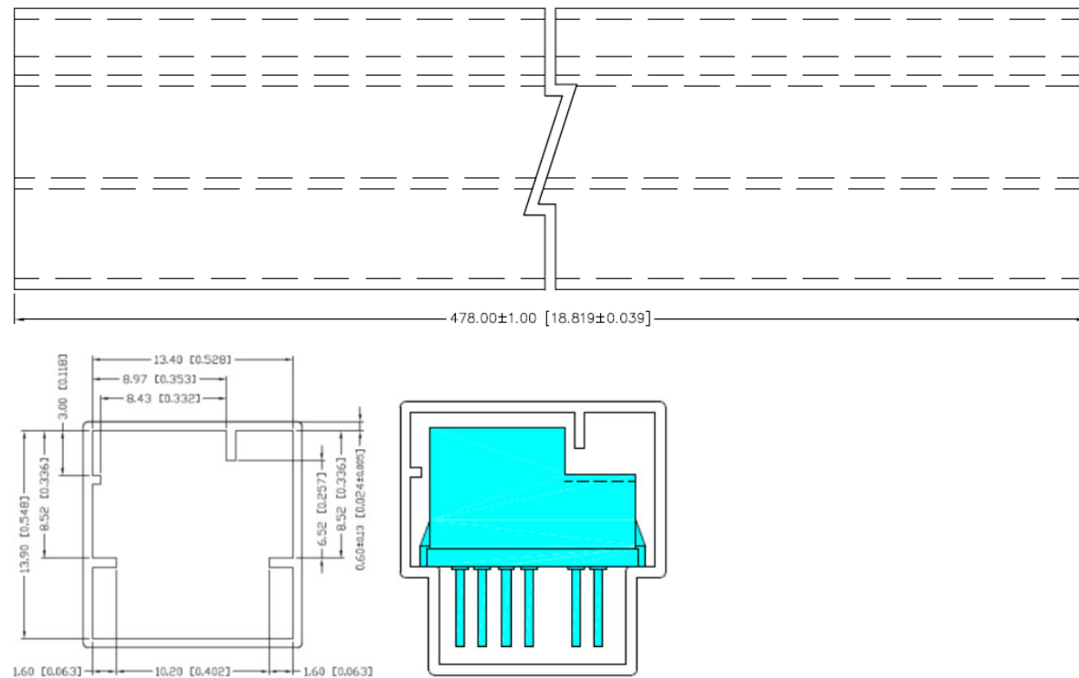
Figure 22: Packing Details
