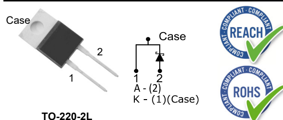
TO-220-2L
