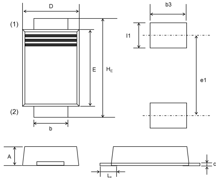
SOD-128, (PMDTM)
