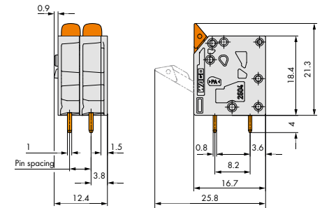
PCB terminal block for power supplies
