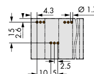
Footprint (top view)
