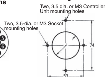
Mounting Holes
