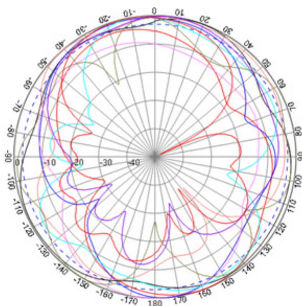
YZ PLANE
